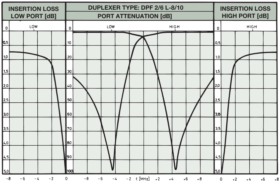
TYPICAL RESPONSE CURVES @ 9 MHz DUPLEX SPACING:
