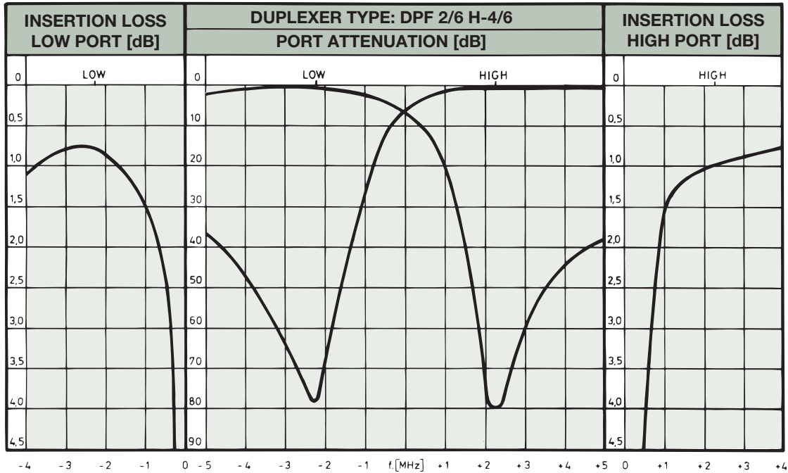
TYPICAL RESPONSE CURVES @ 4.5 MHz DUPLEX SPACING:
